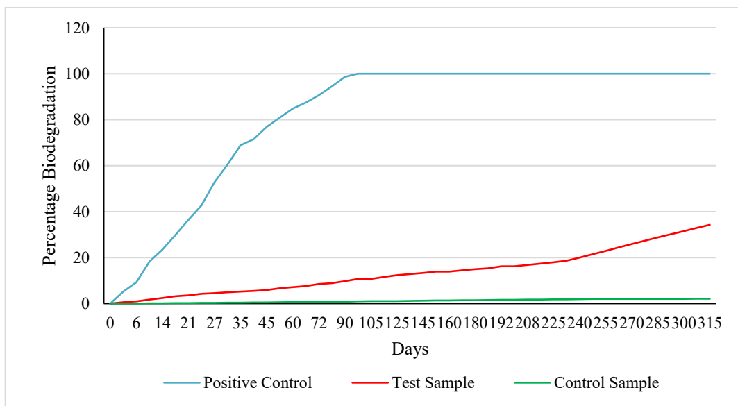
Graph 1: Percentage biodegradation of Positive Control, Test sample and Control sample under aerobic composting
