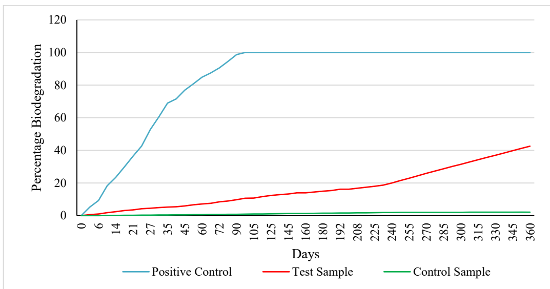
Graph 1: Percentage biodegradation of Positive Control, Test sample and Control sample under aerobic composting
