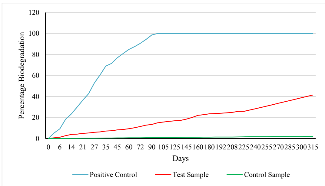
Graph 1: Percentage biodegradation of Positive Control, Test sample and Control sample under aerobic composting
